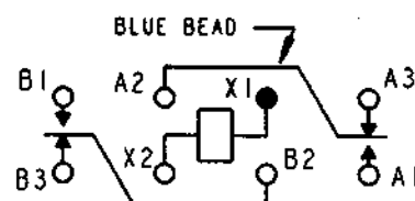
TERMINAL VIEW
