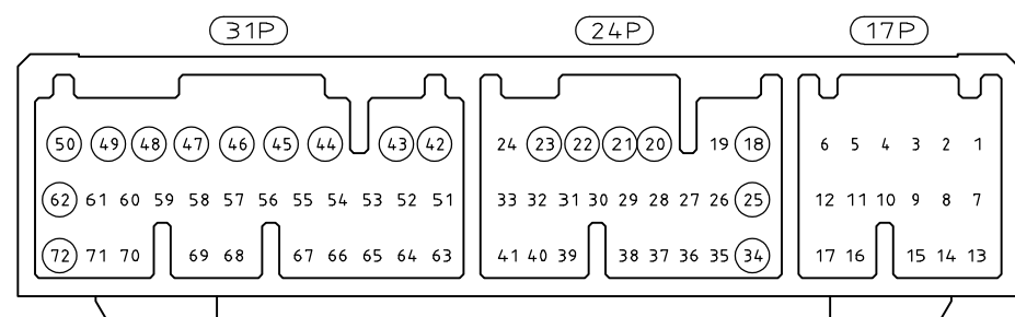
△ FIG 1 CIRCUIT NUMBERS (⊗) ; FOR POWER CIRCUIT (パワー回路用)
