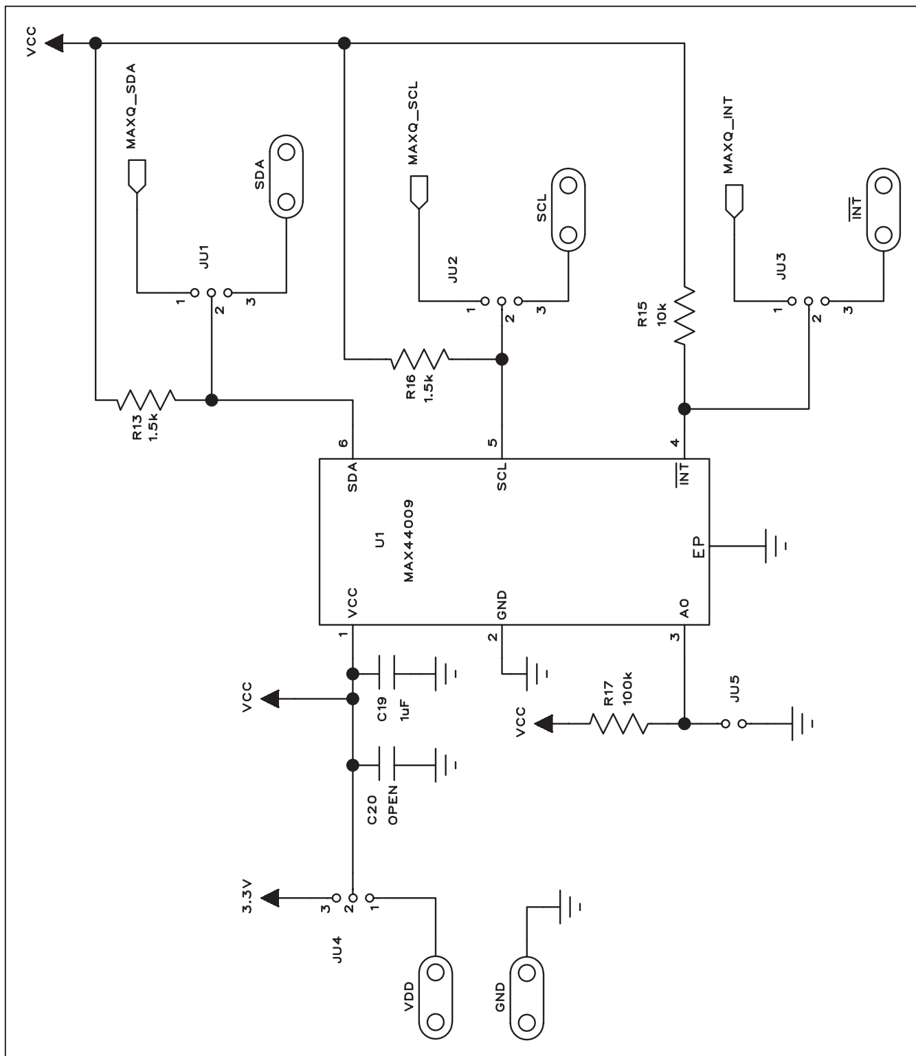
Figure 3a. MAX44009 EV Kit Schematic (Sheet 1 of 2)
