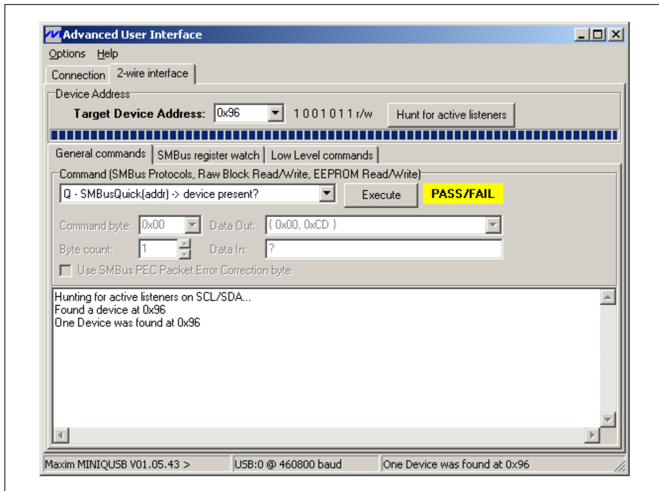
Figure 2. MAX44009 Interface Diagnostic Window
