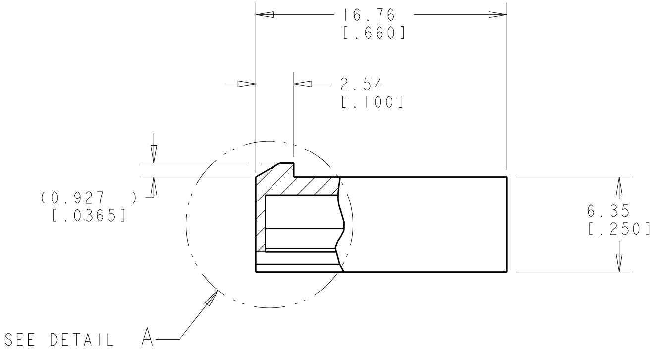
SECTION B-B
