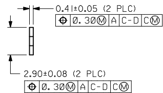
DETAIL Y (BOARD-LOCK)
