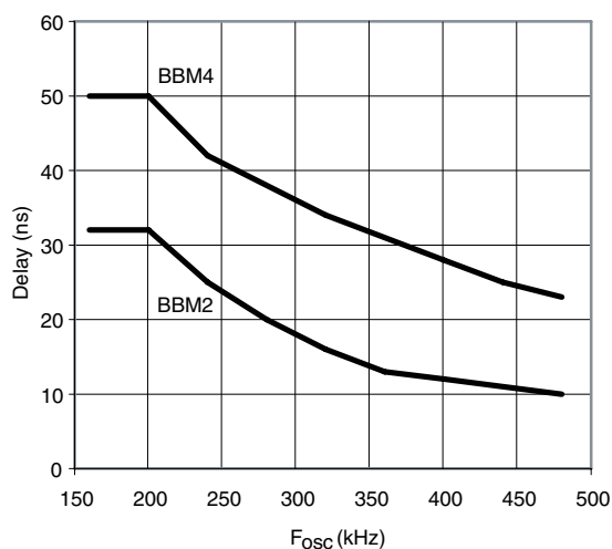
Figure 9. Reduction in t_{BBM2} and t_{BBM4} Si9122E t_{BBM} vs. f_{osc} ; V_{IN} = 50 V, V_{CC} = 10 V, BST = 60 V, LX = 50 V, V_{EP} = 0 V
