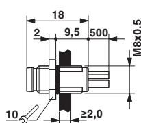
Dimensional drawing
