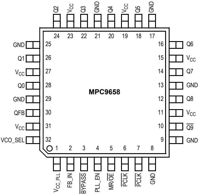
Figure 2. MPC9658 32-Lead Pinout (Top View)
