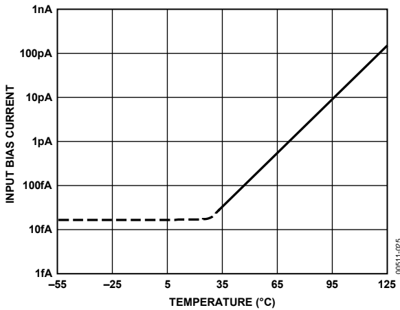
Figure 25. Input Bias Current vs. Ambient Temperature
