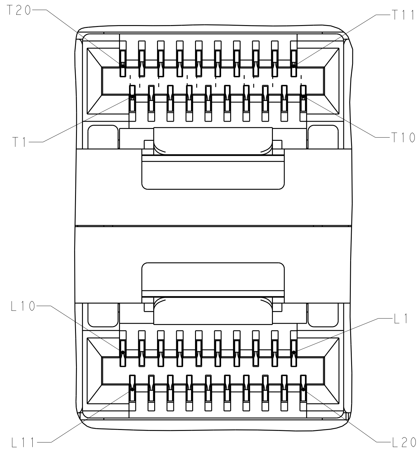
DETAIL A 6X INDIVIDUALLY STACKED SCALE 10:1
