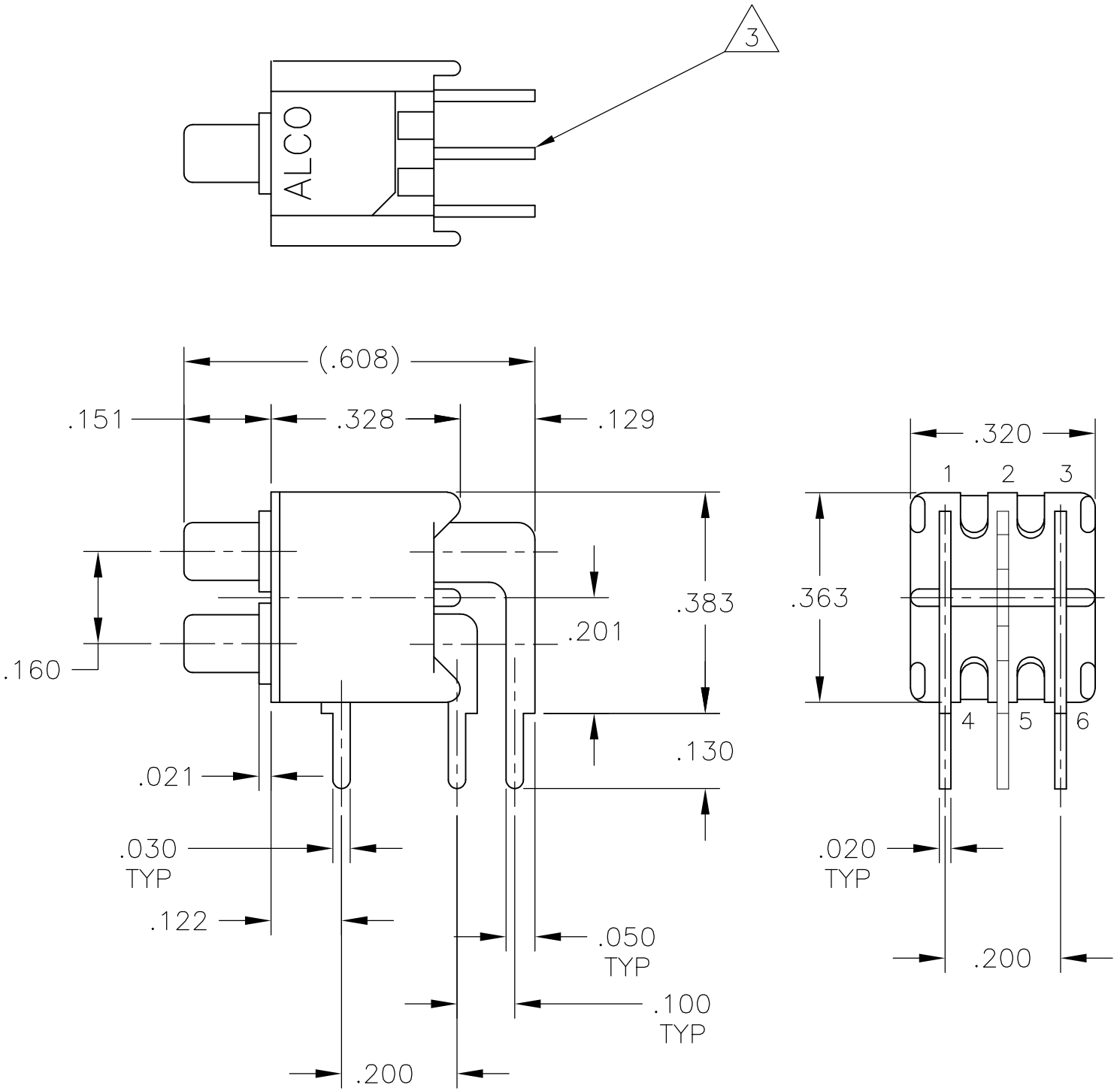
TPA21CCGRA TPA21FFGRA
