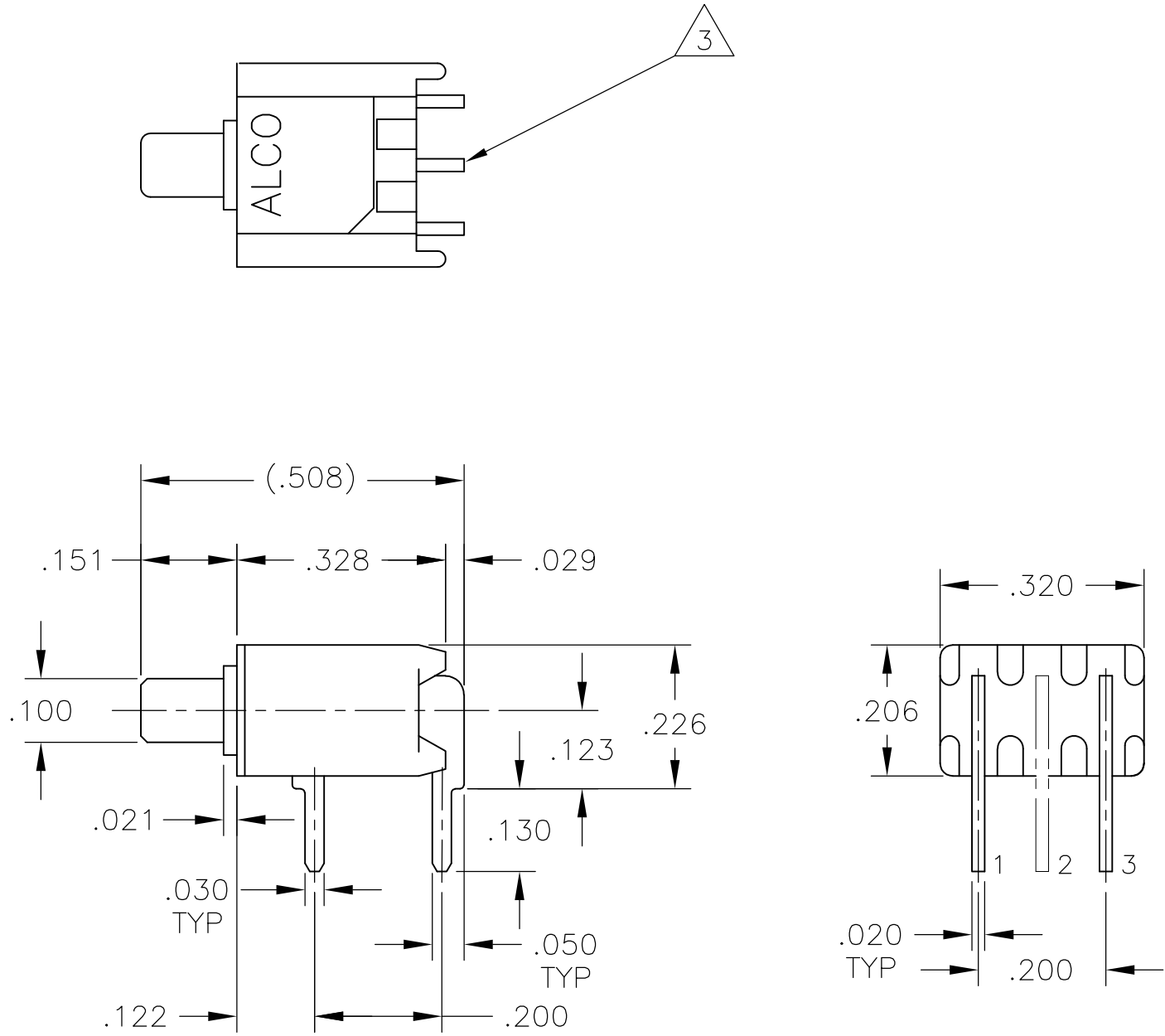
TPA11CGRA TPA11FGRA
