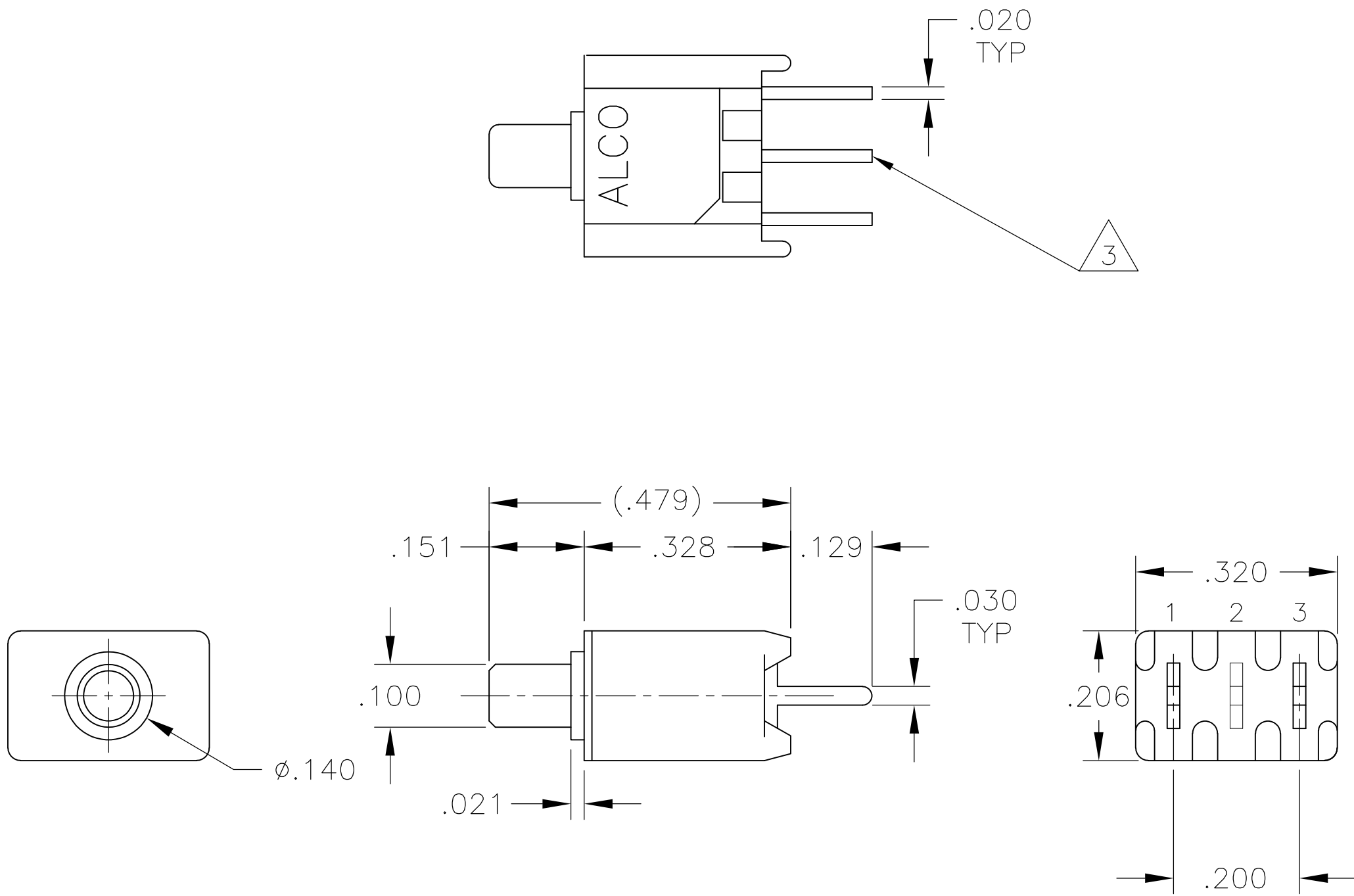
TPA11CGPC TPA11FGPC
