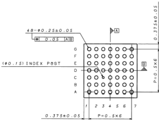
Figure. 64 Package dimensions
