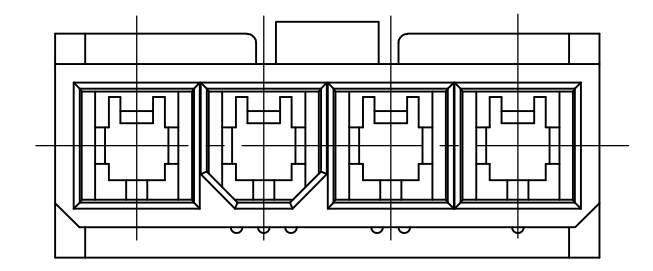
4 POSITION MATING FACE (FOR POLARIZATION IDENTIFICATION)
