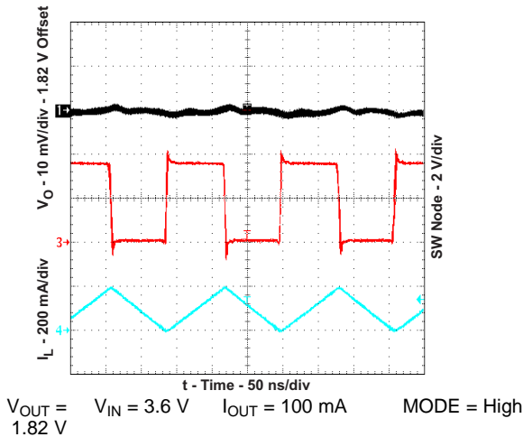
Figure 32. PWM Operation
