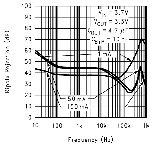
Figure 12. Ripple Rejection
