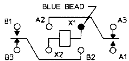
TERMINAL VIEW
