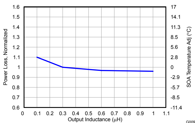
Figure 15. Normalized Power Loss vs Output Inductance
