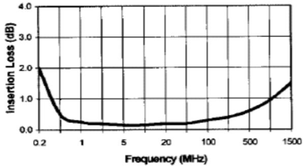
Insertion Loss
