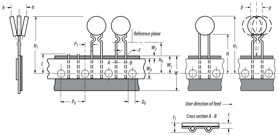
Taped Component Dimensions - per EIA Mark - Figure 1
