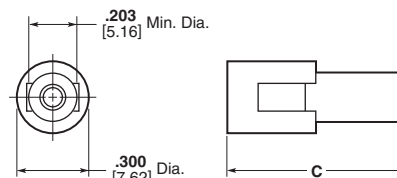
Plug
