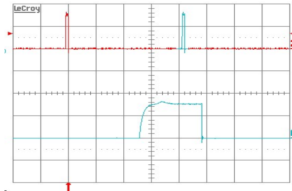
Figure 14. Load current (top trace, 20 A/div., 50 ms/div.) into a 10 m \Omega short circuit during restart, at V_{in} = 48 V. Bottom trace (20 A/div., 2 ms/div.) is an expansion of the on-time portion of the top trace
