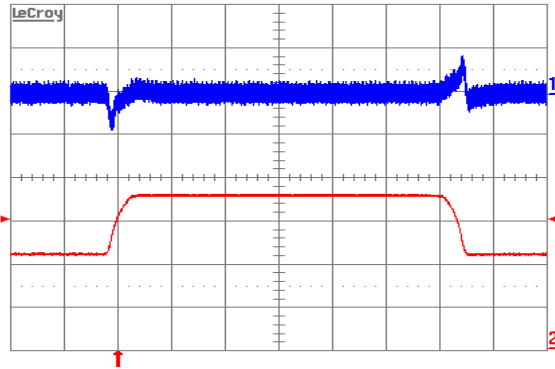
Figure 7. Output voltage response to load current step (12.5 A–18.75 A–12.5 A) at V_{in} = 48 V. Top trace: output voltage (50 mV/div.). Bottom trace: load current (5 A/div.). Current slew rate: 0.1 A/ \mu s. C_o = 1 \mu F ceramic + 10 \mu F tantalum. Time scale: 0.2 ms/div.
