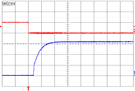
Figure 5. Turn-on transient at full rated load current (resistive) with no output capacitor at V_{in} = 48 V, triggered via ON/OFF pin. Top trace: ON/OFF signal (5 V/div.). Bottom trace: Output voltage (1.0 V/div.). Time scale: 2 ms/div.
