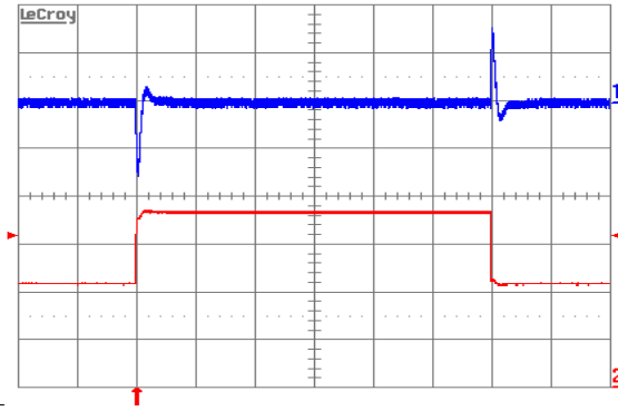
Figure 8. Output voltage response to load current step (12.5 A–18.75 A–12.5 A) at V_{in} = 48 V. Top trace: output voltage (100 mV/div.). Bottom trace: load current (5 A/div.). Current slew rate: 5 A/ \mu s. C_o = 470 \mu F POS + 1 \mu F ceramic. Time scale: 0.2 ms/div.
