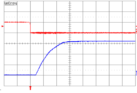
Figure 6. Turn-on transient at full rated load current (resistive) plus 20,000 \mu F at V_{in} = 48 V, triggered via ON/OFF pin. Top trace: ON/OFF signal (5 V/div.). Bottom trace: Output voltage (1 V/div.). Time scale: 2 ms/div.
