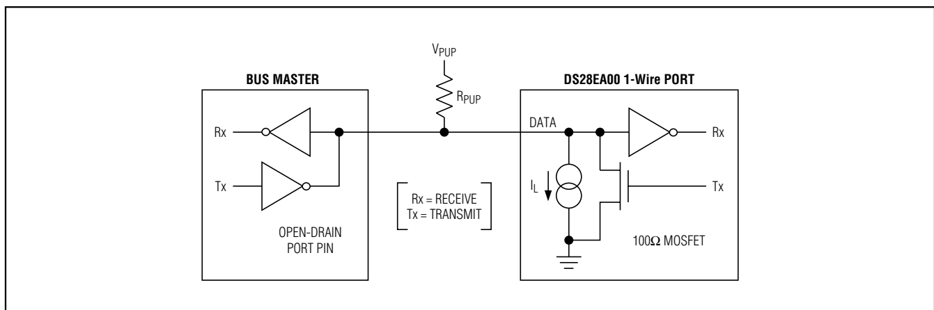
Figure 10. Hardware Configuration
