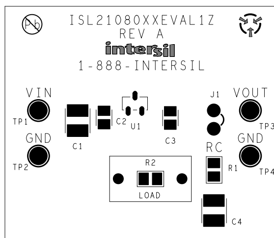
FIGURE 4. ASSEMBLY DRAWING
