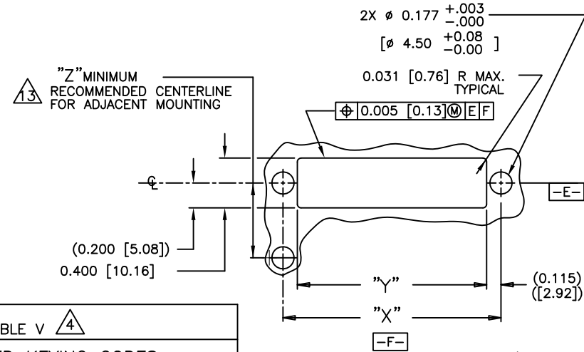
RECOMMENDED PANEL CUT-OUT 12 FIGURE 1
