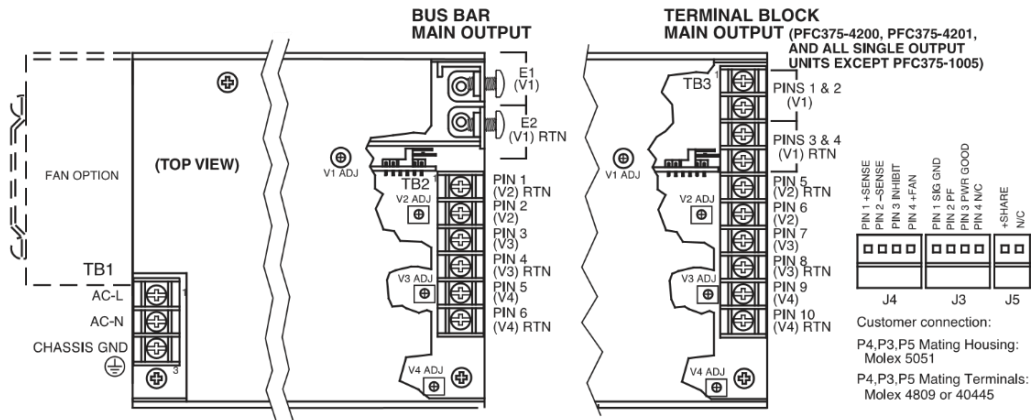
Figure 1. Mechanical Drawing PFC375
