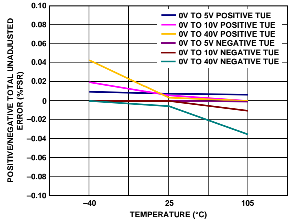
Figure 8. Total Unadjusted Error vs. Temperature
