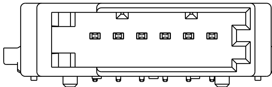
KEYING CODE "C" SCALE 4:1
