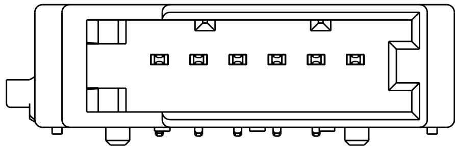
KEYING CODE "D" SCALE 4:1
