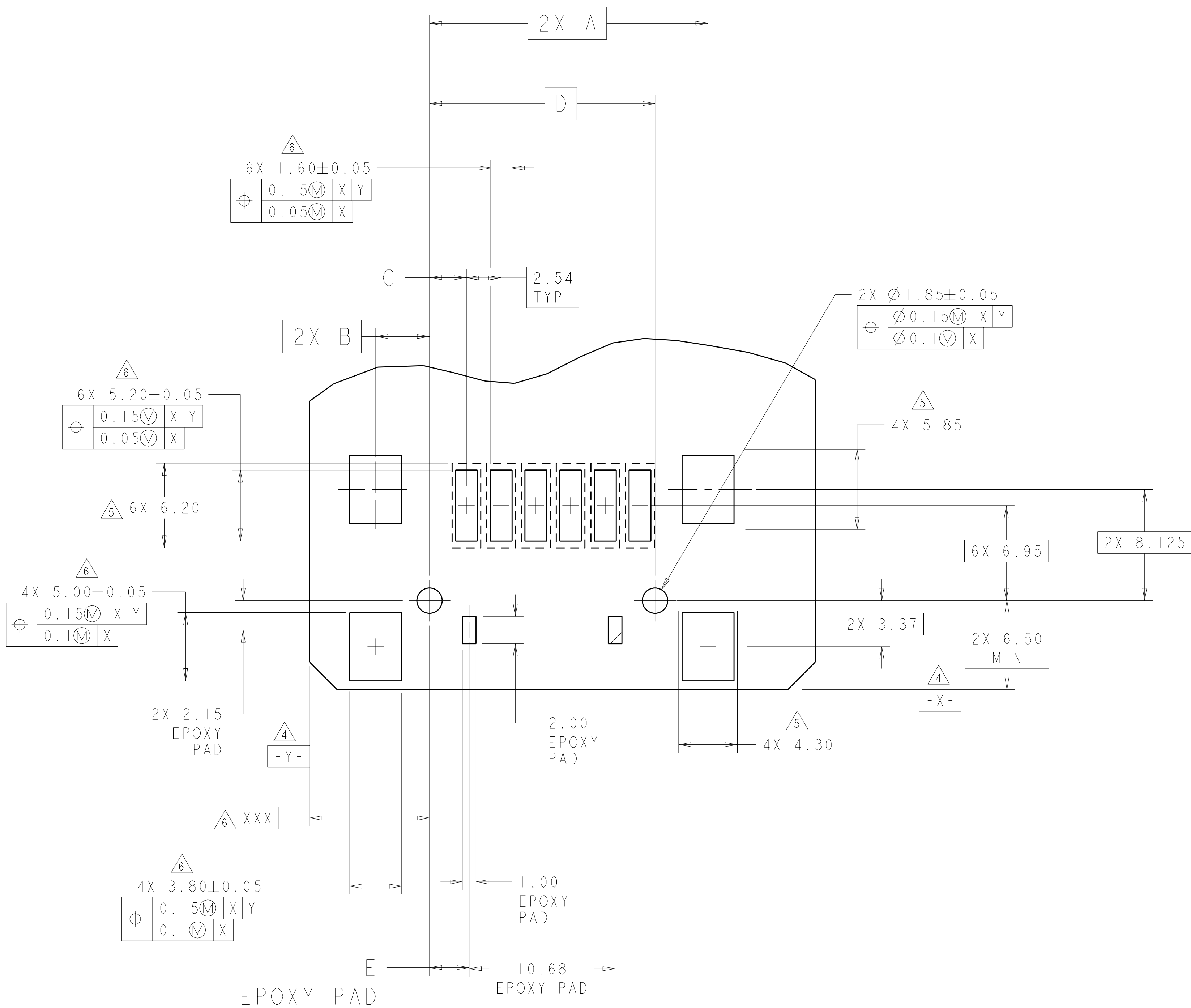
RECOMMENDED PC BOARD LAYOUT CONNECTOR SIDE OF BOARD SCALE 5:1
