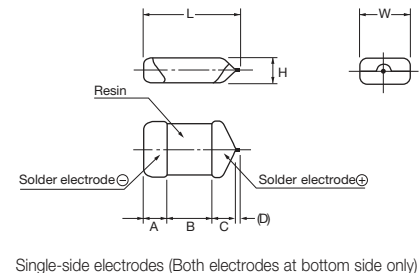
Single-side electrodes (Both electrodes at bottom side only)
