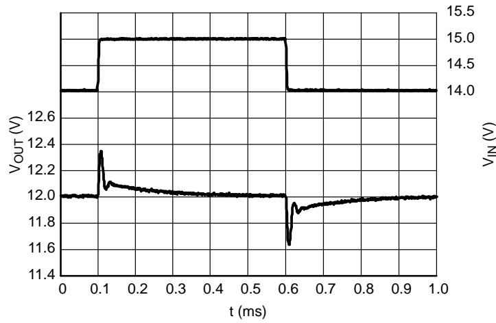
Figure 33. Line Transients, 12.0 V Version, t_R = t_F = 5 \mu\text{s} , I_{OUT} = 30 \text{ mA}
