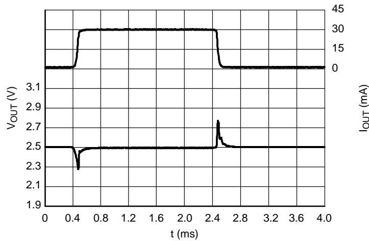
Load Transients, 2.5 V Version, I_{OUT} = 1 - 30 \text{ mA} , t_R = t_F = 50 \mu\text{s} , V_{IN} = 4.5 \text{ V}
