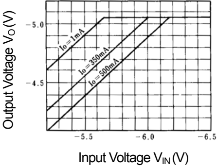
NJM79M05 Dropout Characteristics (T j =25°C)
