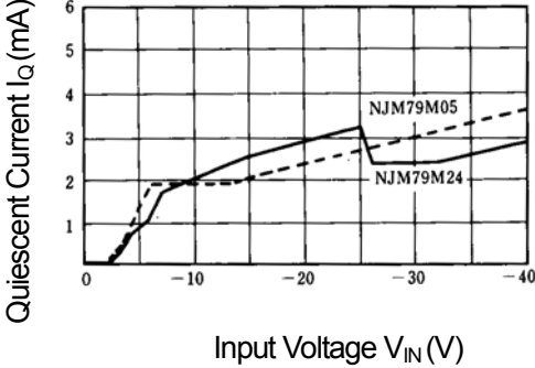
Quiescent Current vs. Input Voltage (T j =25°C, I o =0mA)
