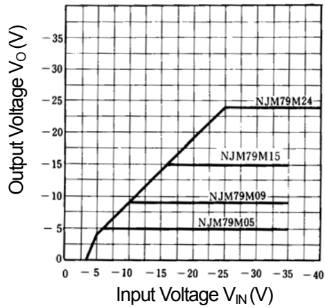
NJM79M00 Output Characteristics
