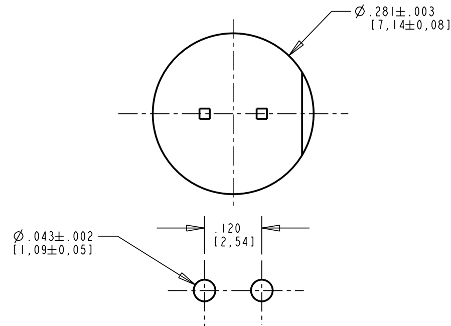
RECOMMENDED P.C.B. HOLE PATTERN
