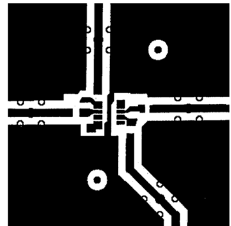
Figure 64. Inverter SOIC Board Layout (Component Layer)
