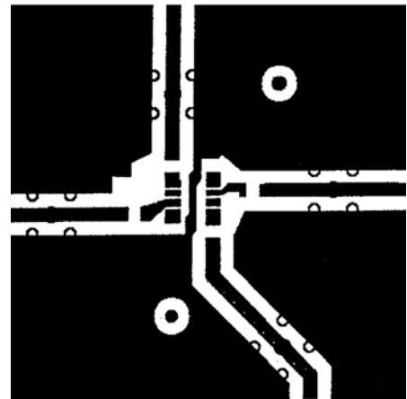
Figure 65. Noninverter SOIC Board Layout (Component Layer)
