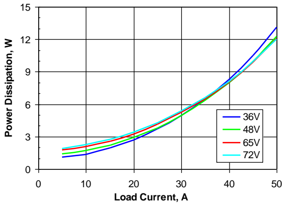
Figure 4. Power dissipation vs. load current and input voltage for SQE48T50012 converter mounted vertically with air flowing from pin 3 to pin 1 at a rate of 300 LFM (1.5 m/s) and T_a = 25\text{ }^\circ\text{C} .
