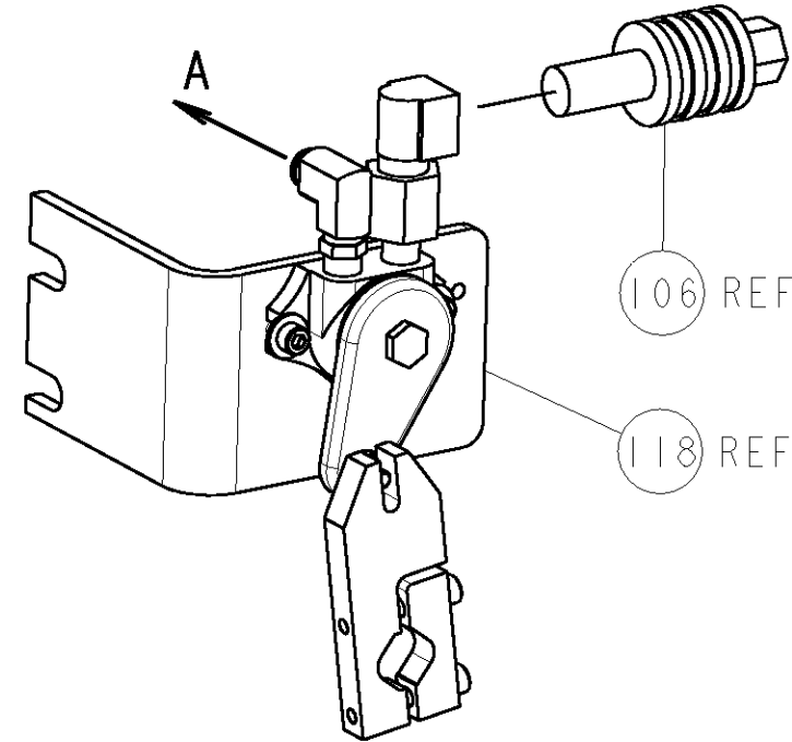
AIR FEED VALVE ASM (-2 ONLY)
