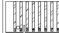
LAYOUT FOR CONNECTOR NO. 0-1740533-9 LAYOUT FOR CONNECTOR NO. 1-1740533-9 (W ITHOUT PAD 9)
