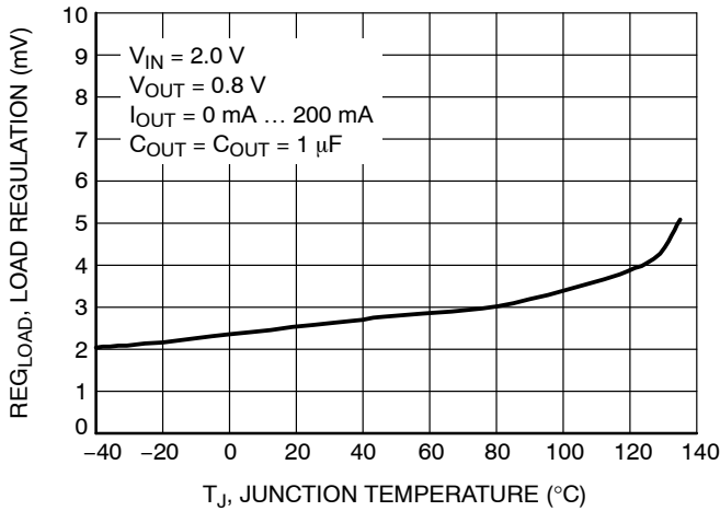
Figure 23. Load Regulation vs. Temperature, V OUT = 0.8 V
