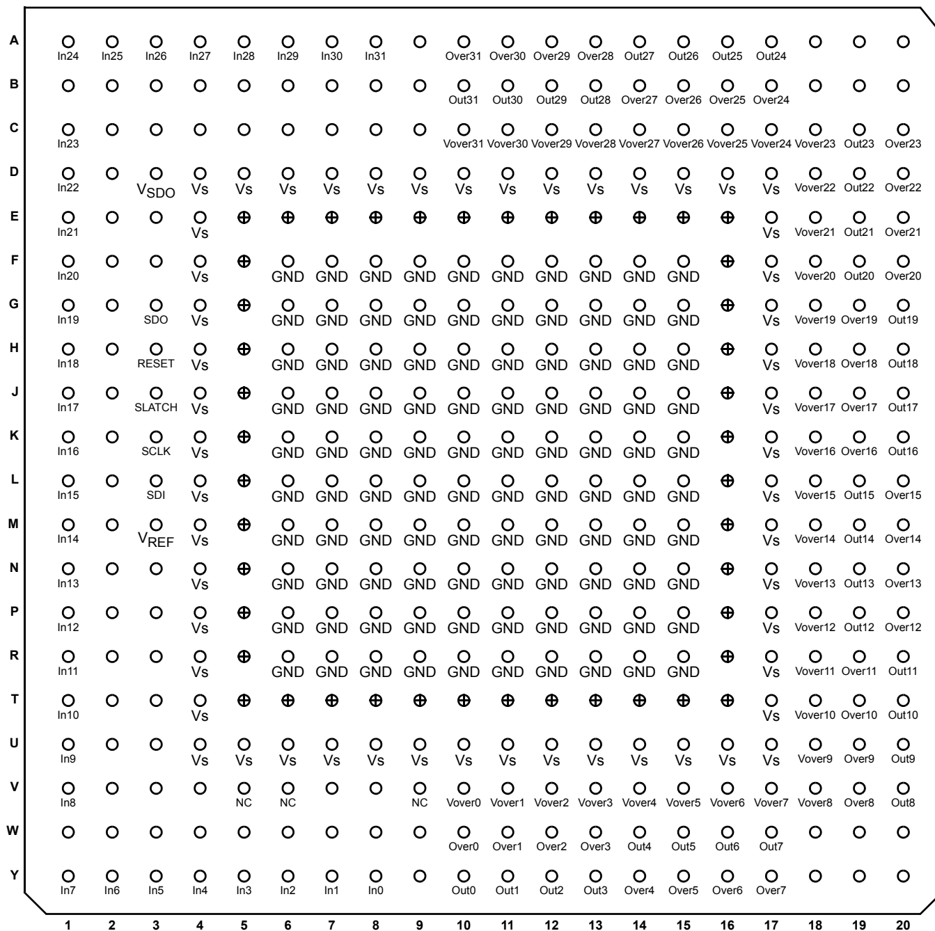
ISL59532 (356 LD HBGA) TOP VIEW
