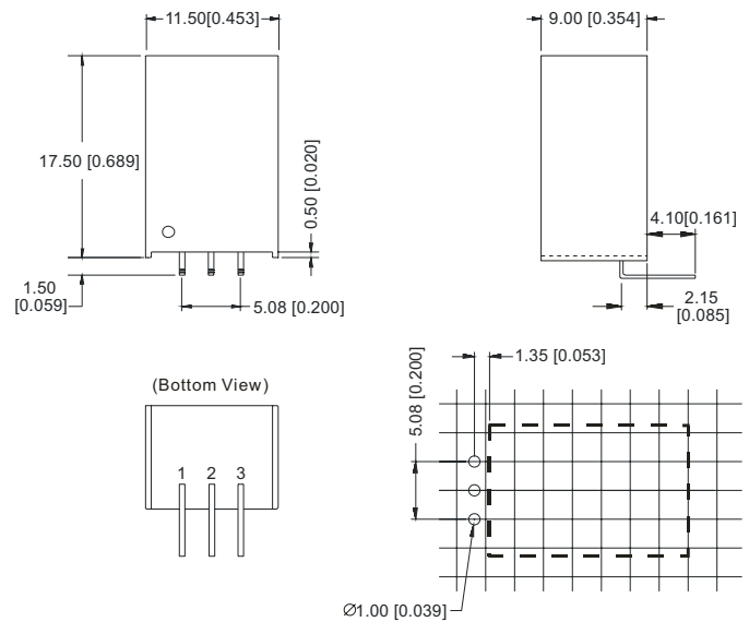
V78XX-1000R
