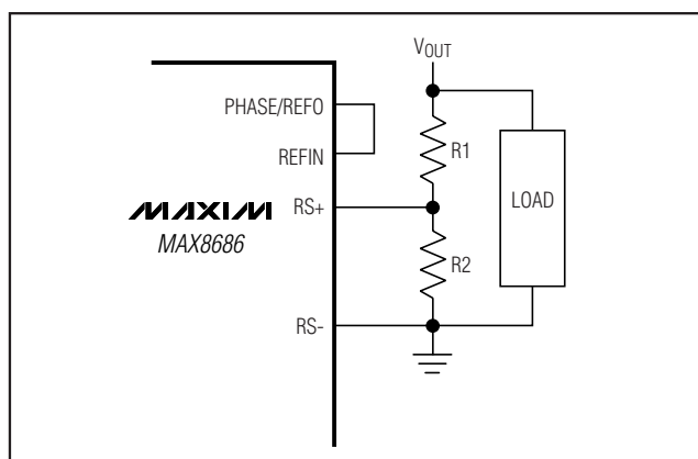
Figure 1b. Output Voltage Above 3.3V
