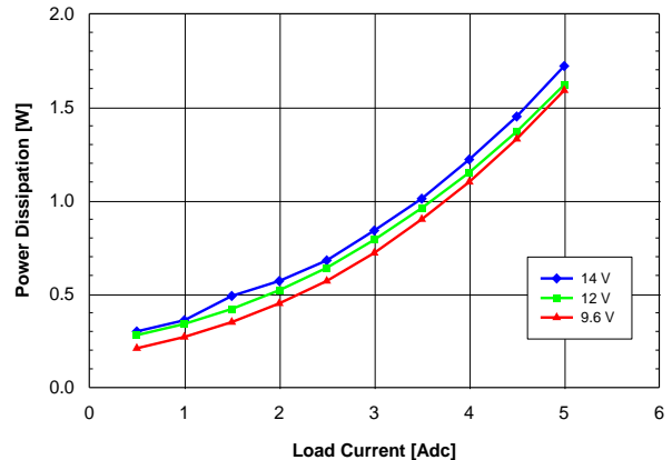
Fig. 1.2V.4: Power Loss vs. load current and input voltage for V_{out} = 1.2V converter mounted vertically with air flowing from pin 5 to pin 1 at a rate of 200 LFM (1 m/s) and T_a = 25^{\circ}C .
