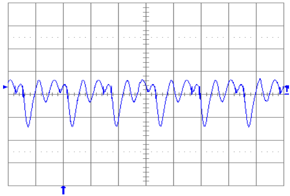
Fig. 1.8V.6: Output voltage ripple (10mv/div) at full rated load current with external capacitance 47\mu F ceramic + 1\mu F ceramic and V_{in} = 12V for V_{out} = 1.8V . Time scale: 2 \mu s /div.
