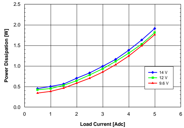
Fig. 2.0V.4: Power Loss vs. load current and input voltage for V_{out} = 2.0V converter mounted vertically with air flowing from pin 5 to pin 1 at a rate of 200 LFM (1 m/s) and T_a = 25^{\circ}\text{C} .
