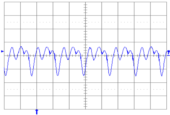
Fig. 2.0V.6: Output voltage ripple (10mv/div) at full rated load current into a resistive load with external capacitance 47\mu\text{F} ceramic + 1\mu\text{F} ceramic and V_{in} = 12V for V_{out} = 2.0V . Time scale: 2 \mu\text{s} /div.
