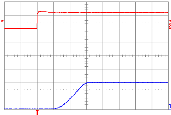
Fig. 2.0V.5: Turn-on transient for V_{out} = 2.0V with application of V_{in} = 12V at full rated load current (resistive) and 47\mu\text{F} external capacitance. Top trace: V_{in} (10V/div); Bottom trace: V_{out} (1V/div); Time scale: 2 ms/div.
