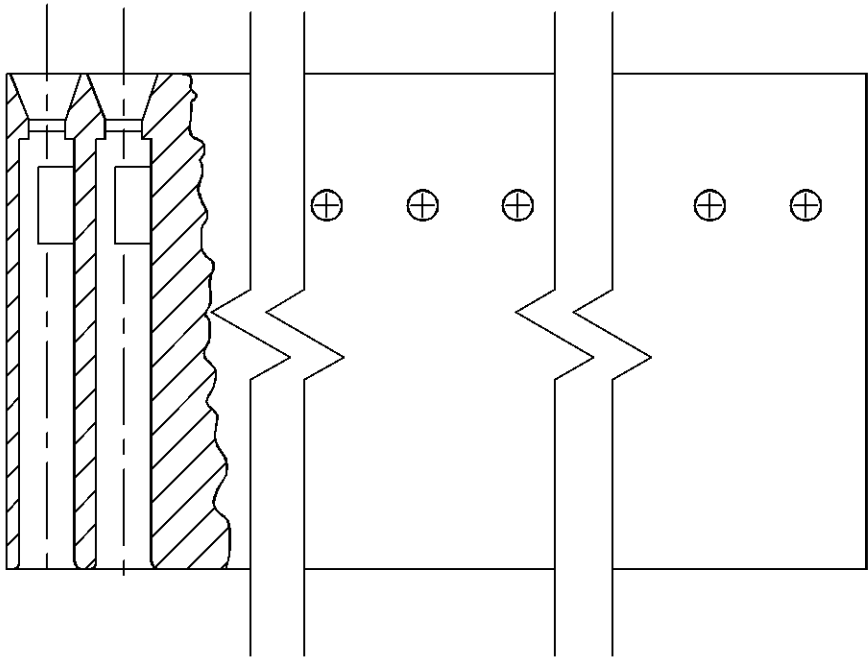
SECT Y-Y
