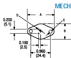
TO-66
