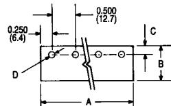
DUAL TO-220
