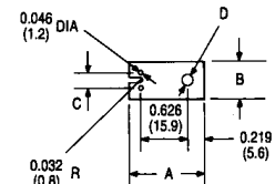
TO-66 (RECTANGLE)
