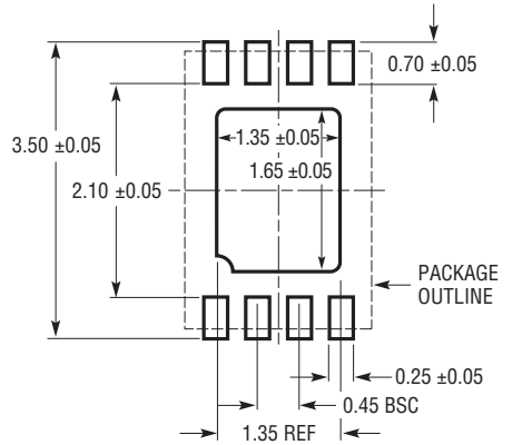
DCB Package 8-Lead Plastic DFN (2mm × 3mm) (Reference LTC DWG # 05-08-1718 Rev A)
