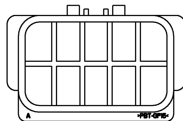
12 POS 2040594-6 SCALE 2:1
