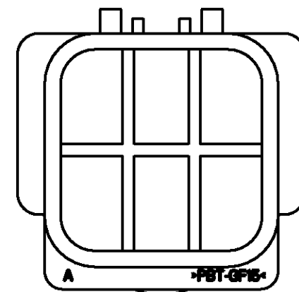
6 POS 2040594-4 SCALE 2:1
