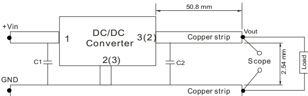
Start-up and Load Transient Response Test
