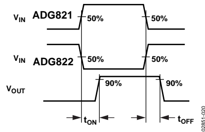
Figure 20. Switching Times
