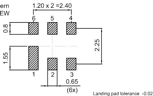
Figure 2: Drawing of package. See Sec. Package information (p. 19).
