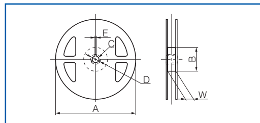
Standard Reel Dimensions
