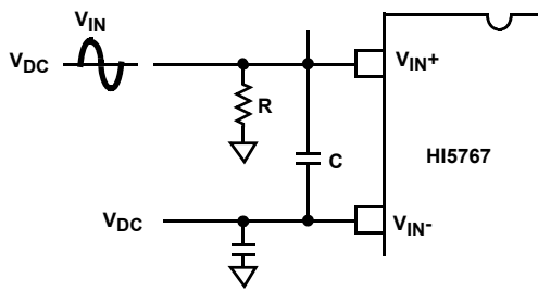
FIGURE 19. DC COUPLED SINGLE ENDED INPUT
