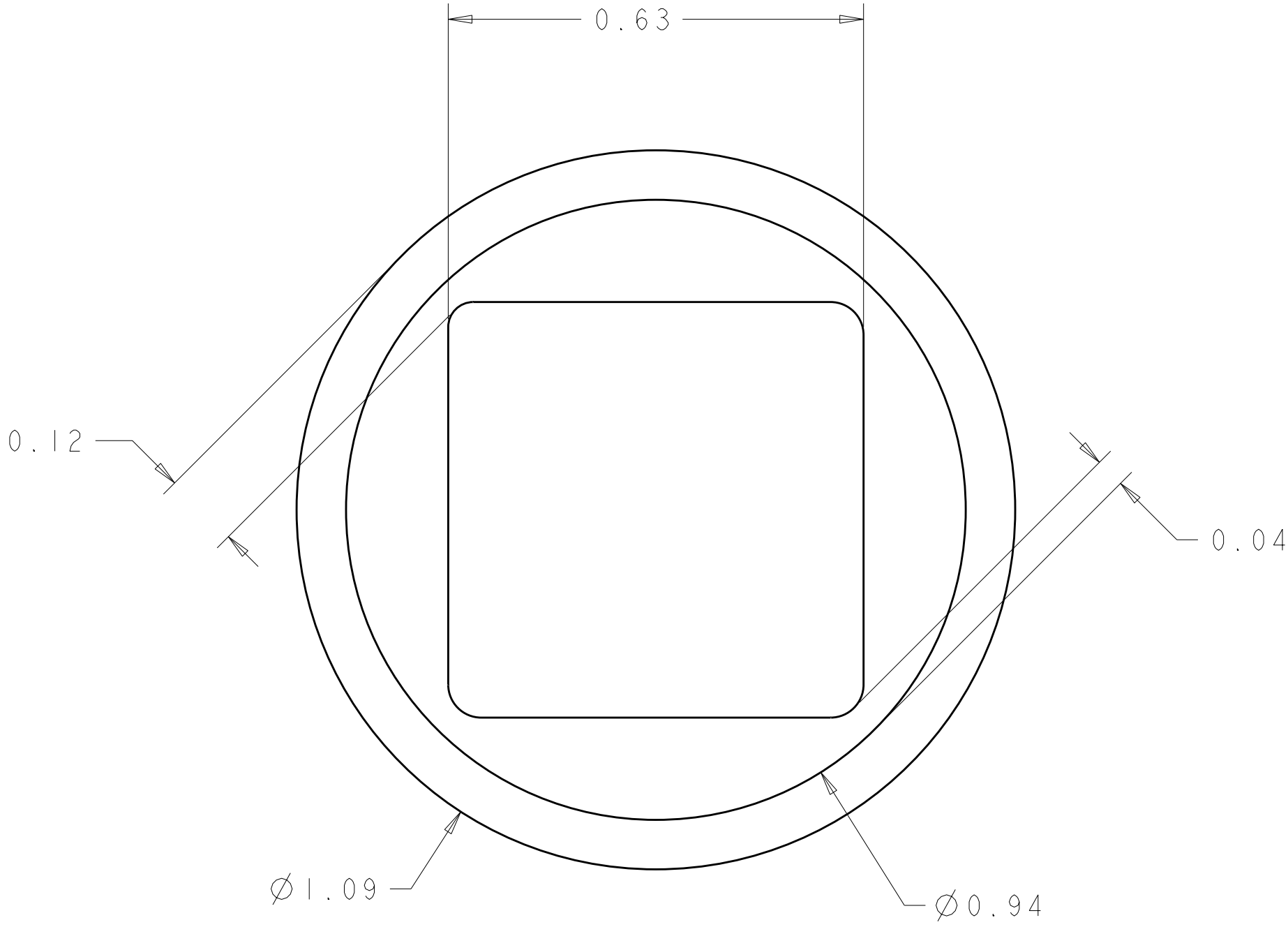
SOLDER TERMNIATION AREA SCALE 40:1 RECOMMENDED PRINTED CIRCUIT SOLDER HOLE FINISHED HOLE: Ø1.02 [.040] ±.08 [.003] DRILLED HOLE: Ø1.15 [.0453] ±.013 [.0005] COPPER PLATE: .025 [.0010] MIN TIN PLATE: .008 [.0003] MIN. (PER SURFACE)
